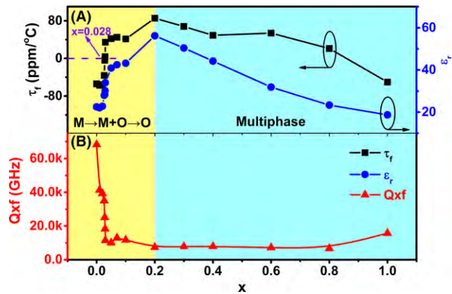
FIGURE 7 Microwave dielectric properties of ZR-x ceramics sintered at their optimal temperatures
