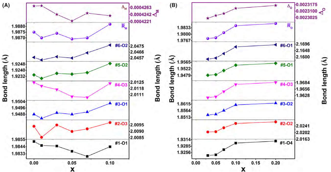
FIGURE 5 Variation in bond length and distortion in octahedra of the (A) M and (B) O phases in ZR- x ceramics
