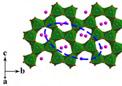
(B) \text{LaTiNbO}_6 (O) Pnma
