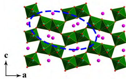
(B) \text{LaTiNbO}_6 (O) Pnma
