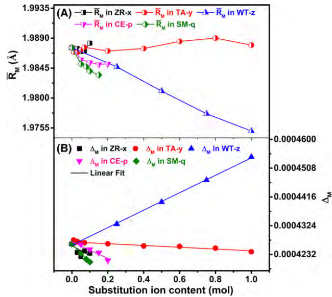
FIGURE 6 (A) The average bond length and (B) the distortion of M-phase octahedra in ZR-x, TA-y, WT-z, CE-p and SM-q ceramics as indicated
